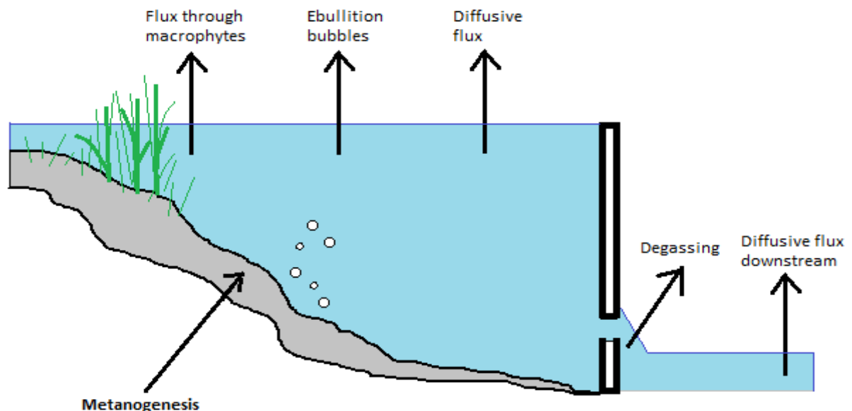
Figure 1 The different pathways of \text{CH}_4 emissions connected to hydroelectric reservoirs.
