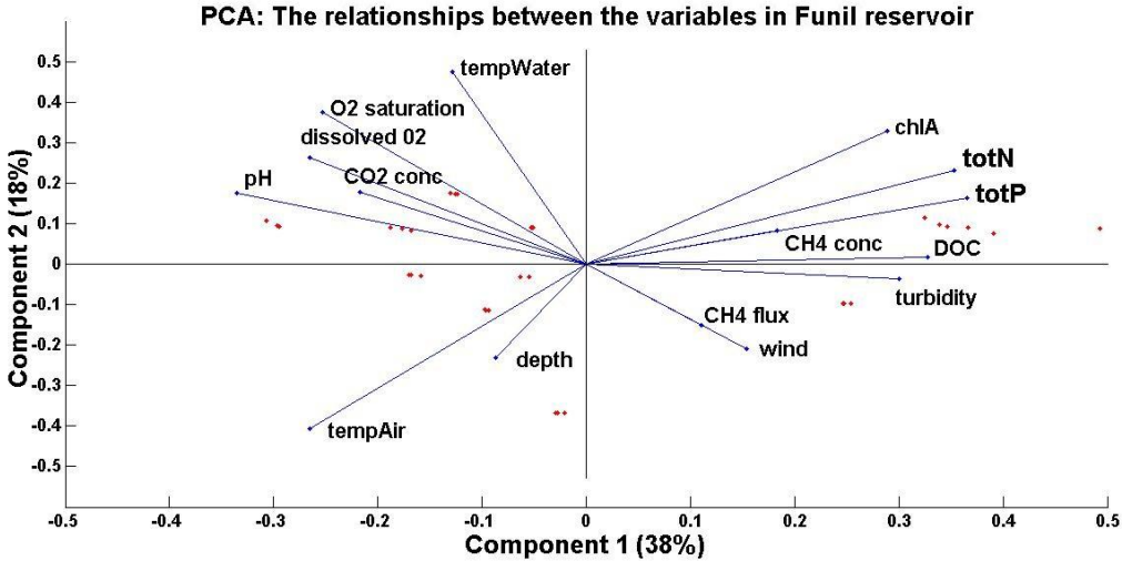
Figure 16 PCA of Funil with 15 variables.
