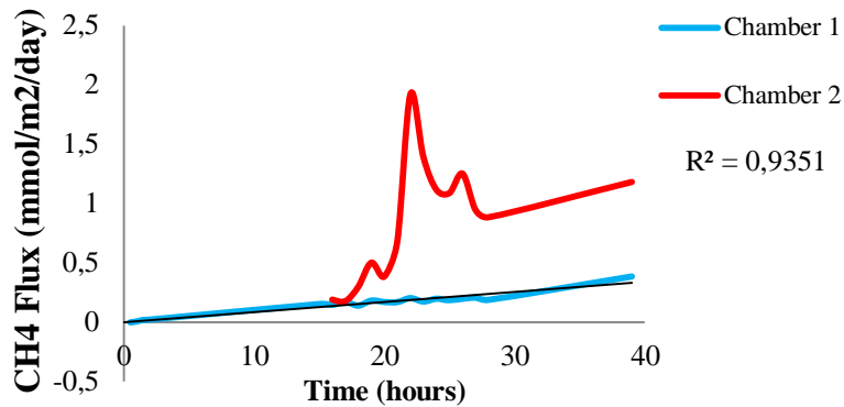
Figure 13 Temporal measurements of CH 4 flux in Três Marias during 36 hours deployment time from two chambers next to each other
