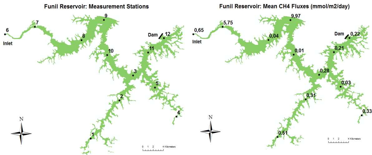
Figure 7 Funil reservoir: measurement stations and their mean CH 4 fluxes after 30 minutes deployment time.
