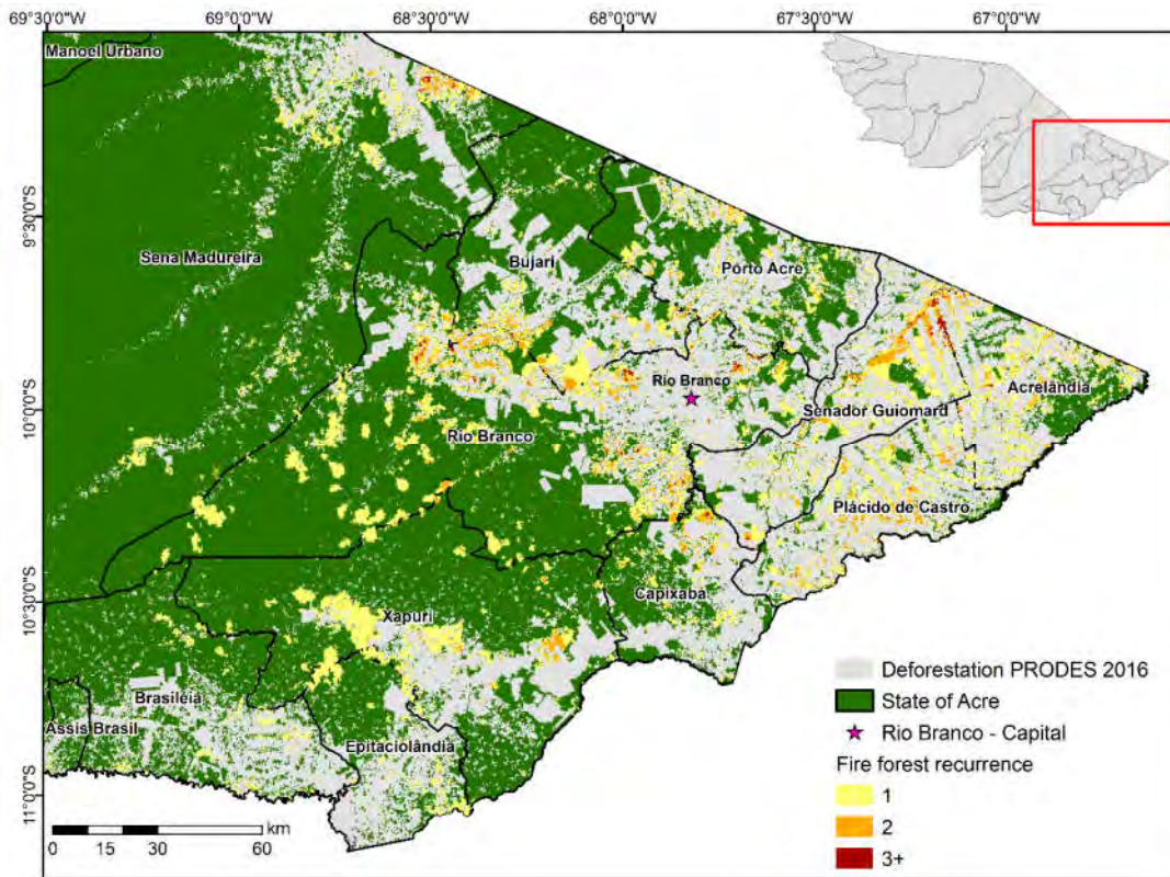
Figure 9. Forest-fire scars of areas burned one, two and three or more times in eastern Acre, Brazil between 1984 and 2016.
