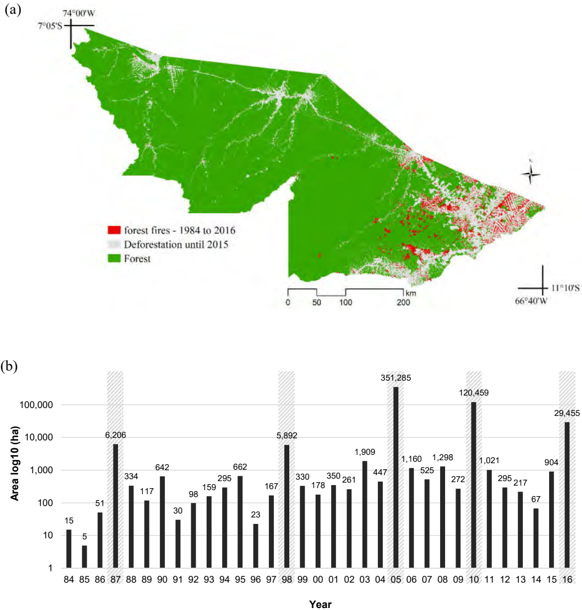
Figure 4. Historical series of forest fires for the state of Acre for the period from 1984 to 2016. (a) Spatial distribution of fires and (b) Temporal distribution of the annual area of occurrence of forest fires, where the cross-hatched bars indicate years of extreme drought from El Niño and/or anomalous warming of the tropical North Atlantic Ocean (Atlantic dipole).
