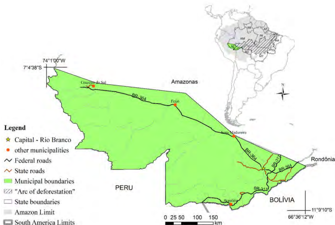
Figure 1. Location of the study area, Acre state, Brazil.
