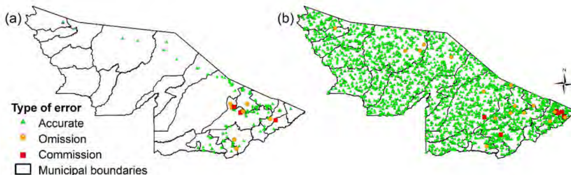
Figure 3. Location of (a) validation points in the field and (b) random points of forest-fire scars.
