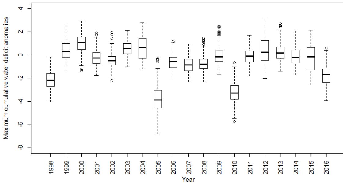
Figure 5. Boxplots of MCWD (maximum cumulative water deficit) for the state of Acre from 1998 to 2016.
