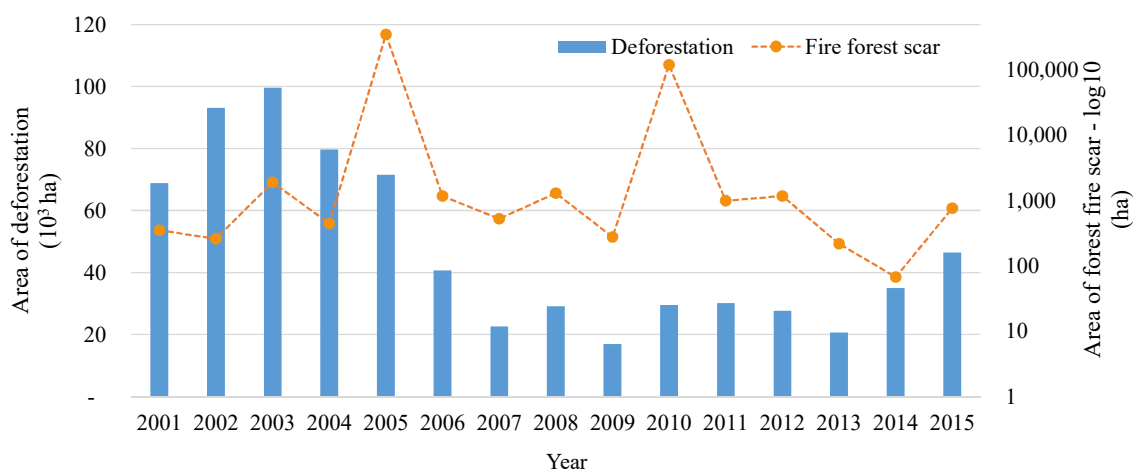
Figure 7. Annual rates of deforestation from PRODES (INPE's Amazon Monitoring Project) and area of annual forest fires in the state of Acre. Note that the "year" for PRODES is from 1 August of the previous year to 31 July of the reported year, while the "year" for forest fires is from 1 January to 31 December.
