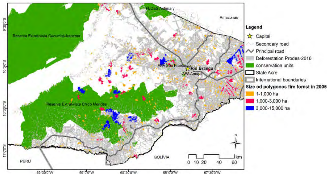
Figure 10. Example of the fires of 2005, size of polygons of forest fires in conservation units under strong anthropic pressure, eastern Acre state, Brazil.
