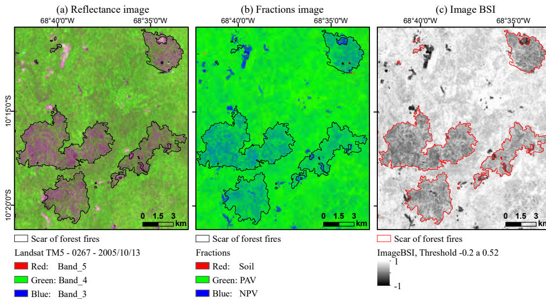
Figure 2. Example of (a) reflectance, (b) fractions and (c) Burn-scar index (BSI) in a Landsat TM5 image from 13 October 2005, Path 002, Row 067.
