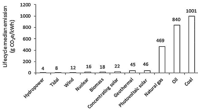
Fig. 1 – Lifecycle median emissions of different sources of electricity according to the IPCC Special Report on Renewable Energy Sources and Climate Change Mitigation (data for 50% percentile from Moomaw et al., 2012, p. 982).
