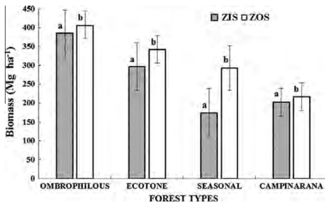
Fig. 5. Total biomass (live + dead; above- and belowground) distinguished by forest group and climatic zone in Roraima (Mg ha -1 ± SD): ZIS = zone with influence of savanna (with shading); ZOS = zone without savanna influence (no shading). Different lowercase letters represent significant differences between means tested in the two zones (Mann-Whitney; 95%).
