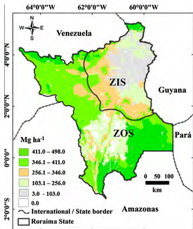
Fig. 4. Reference map of the distribution of biomass (Mg ha -1 ) in the state of Roraima generated by Kriging for external drift (KED). (0–3): areas without data; (3–103): biomass of savanna in the northeastern portion of the state and in neighboring areas in ecotones between dense and open vegetation types; (103.1–256.0) campinarana areas in the south-central portion of the state surrounding areas that are seasonally flooded (for which there are no data), contact areas between campinarana , dense forest, open forest and savanna, in the east-central portion of the state, and ecotones between tropical forest and savanna and between ombrophilous forest and open and dense forest in the north and northeast portions of the state; (256.1–346.0) represent the distribution of biomass of ecotone forests in the southern portion of the state (along the Rio Branco) and of ecotones in the center-north portion of the state between open ombrophilous forest towards the northwest and savanna areas to the east; (346.1–411.0) represents predominantly open ombrophilous forest that is distributed over much of the state and (411.0–498.0) represents dense ombrophilous forest that predominantly occupies the southern and southeastern portions of the state and a few patches in the northernmost portion of the state.
